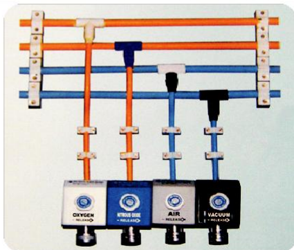
Oxygen Pipeline
